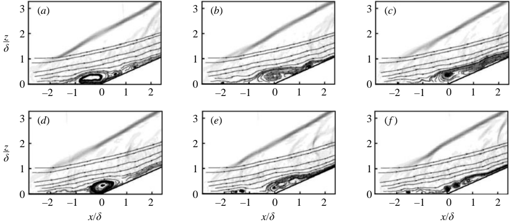
FIGURE 11. Streamlines in (x, z) -planes showing breakdown of the separation bubble. Pressure gradient contours showing the shock location. Time intervals are about 1\delta/U_\infty .
